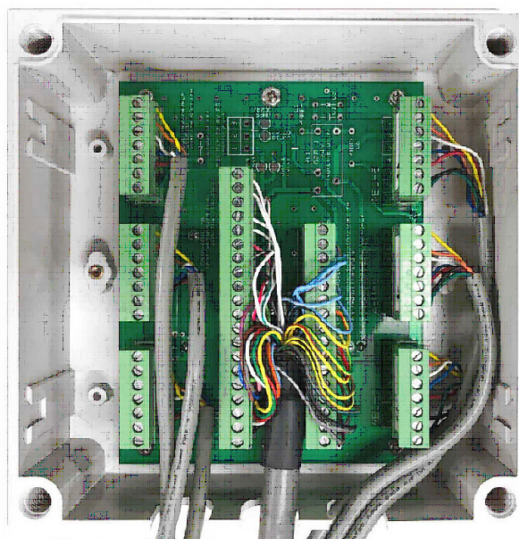
Figure 14 : The inside photograph of Junction Box (3elementtoS mode)
