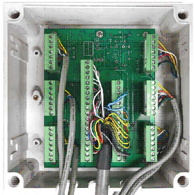
Figure 14 : The inside photograph of Junction Box (3elementtoS modele)
