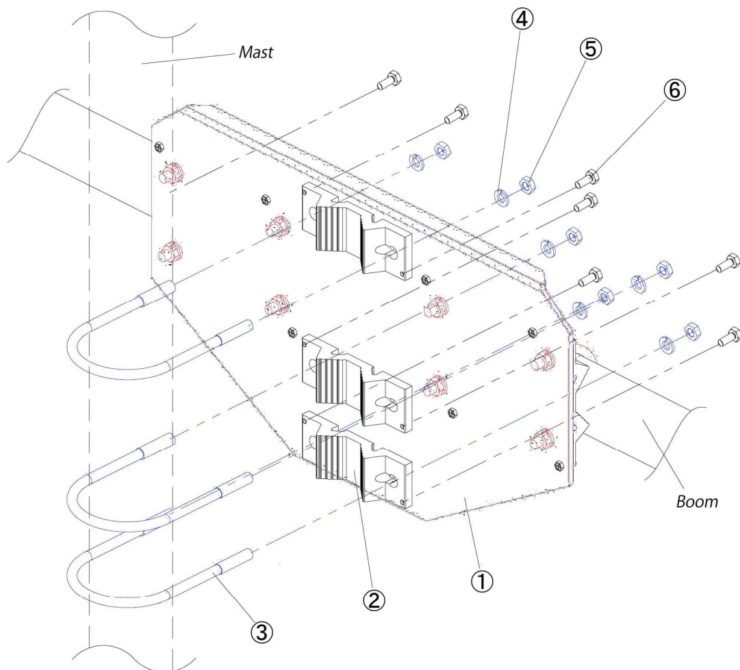
Figure13: Installing the Boom to the Mast.
