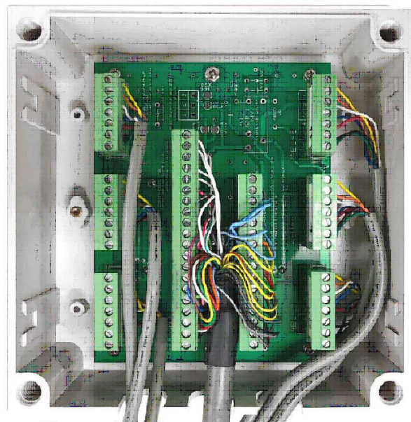
Figure11: The inside photograph of Junction Box (3 elements model).
