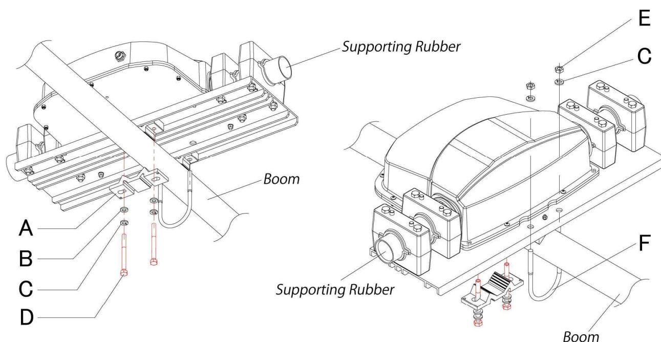
Figure4 (The figure seen from the bottom of AEU)
