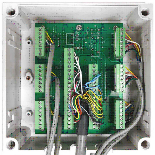
Figure 14 : The inside photograph of Junction Box (3elemerntoS modele)
